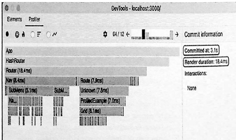
Fig.1. React Profiler: Flame Chart
